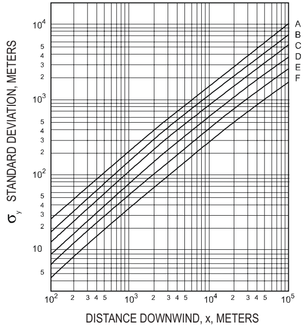
HORIZONTAL STANDARD DEVIATIONS OF A PLUME
