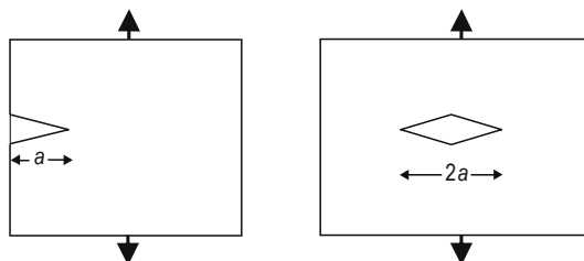
EXTERIOR CRACK ( Y = 1.1 )
