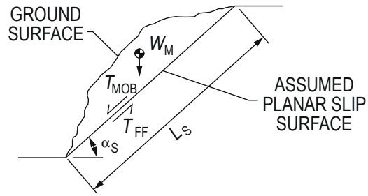
SLOPE FAILURE ALONG PLANAR SURFACE
