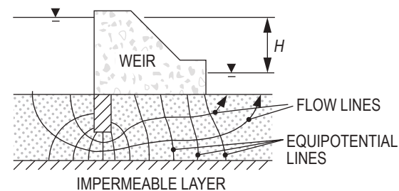
FLOW NET
